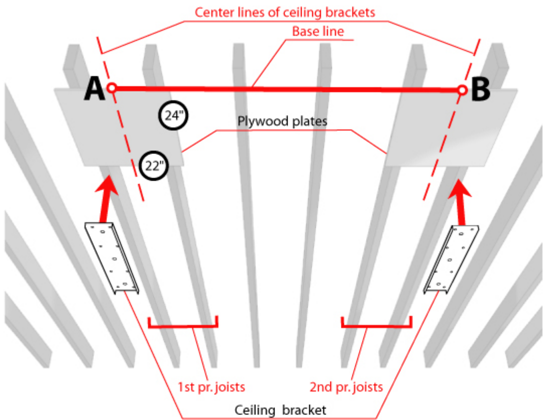
Basic Length (center to center of brackets)
