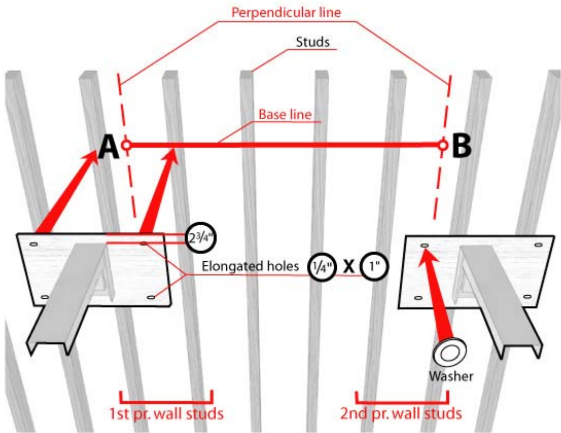
Basic Length (outside edge to outside edge of wall brackets)
